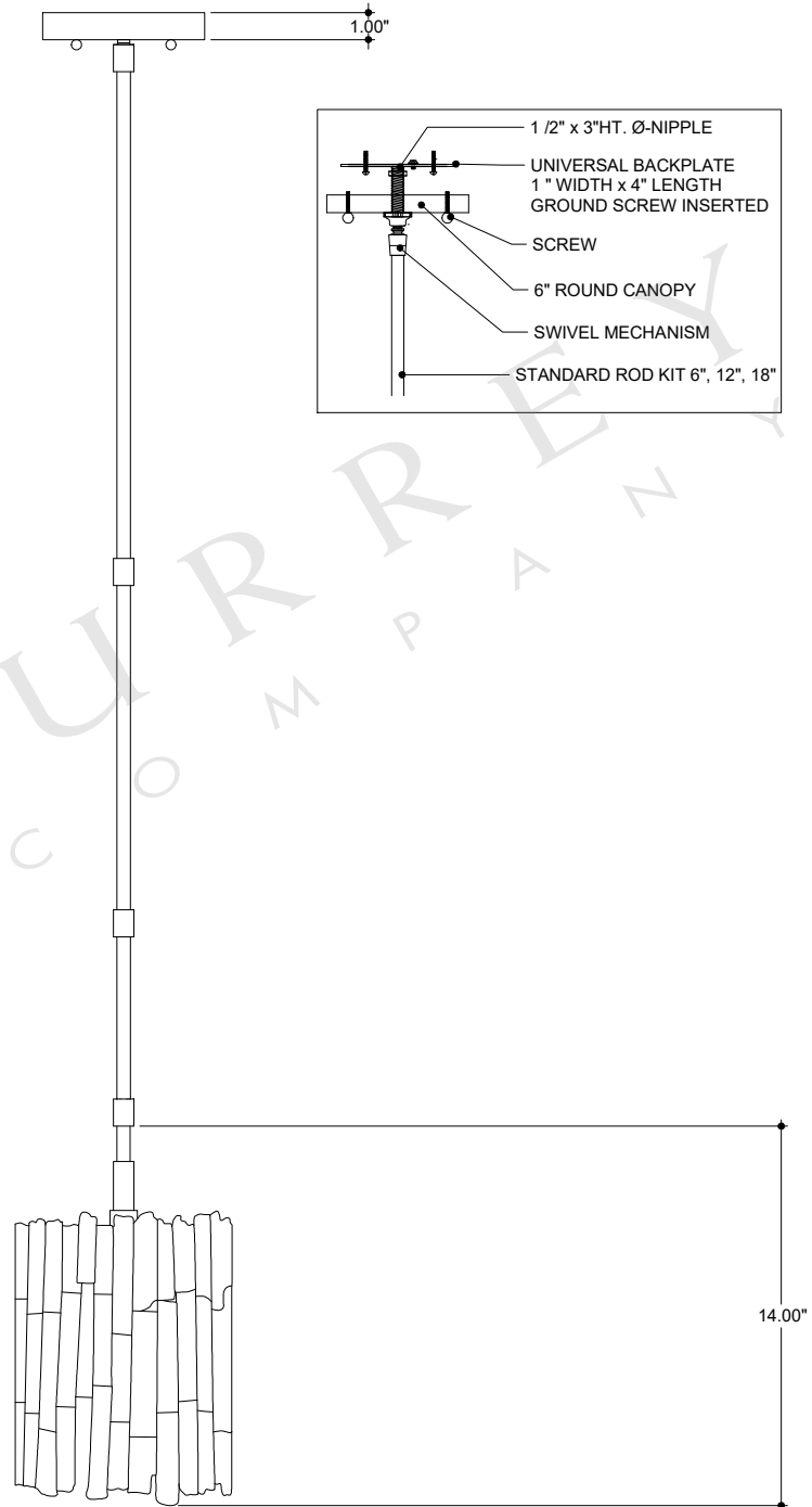
FRONT VIEW
