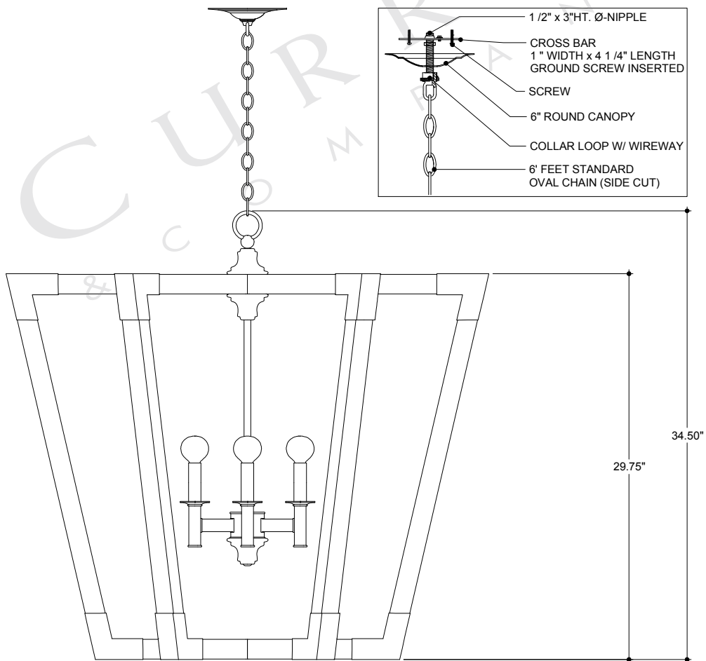
FRONT VIEW
