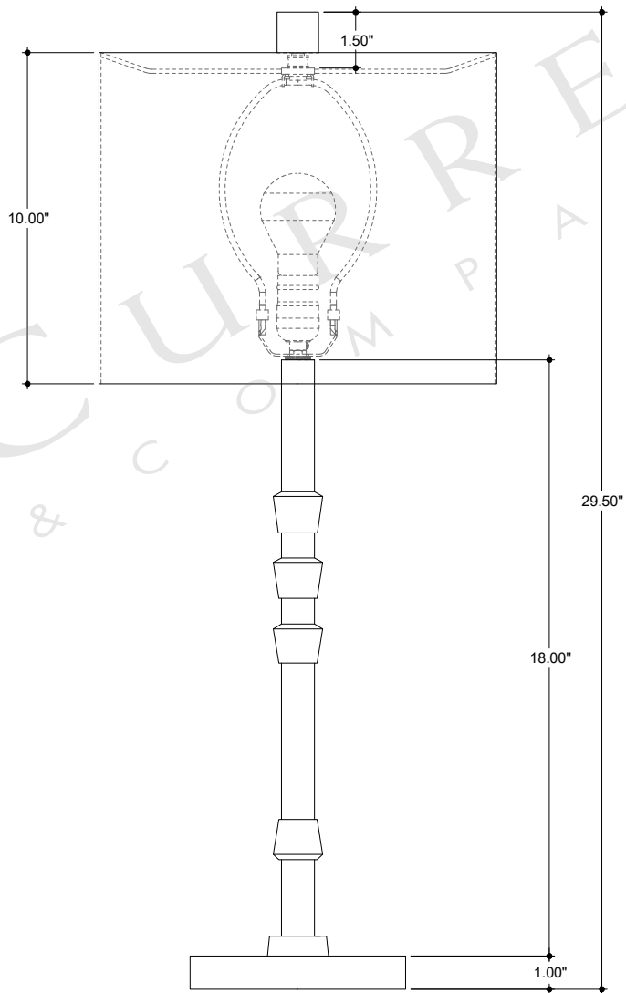
FRONT VIEW
